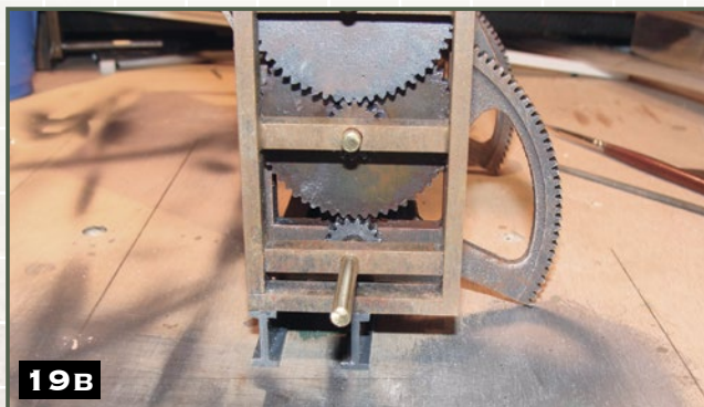
Step 19) Paint and glue the gears. Paint the gears in the same fashion and fit them to the bridge. The lower shaft should stick out from the bridge about 3" on the near side and 1" on the far side. Slide and glue small gears into place on the lower shaft, being careful to avoid getting glue on the gear towers. Slide and glue small gears onto the top shaft so that they line up with the large gears on the bridge. Paint and slide the two remaining gear towers into place.
