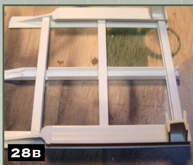
Step 28) Build the ramps. Measure the bridge for its elevation. Build a frame from plastic I-beams. Add some tiling to the base with thin card.
