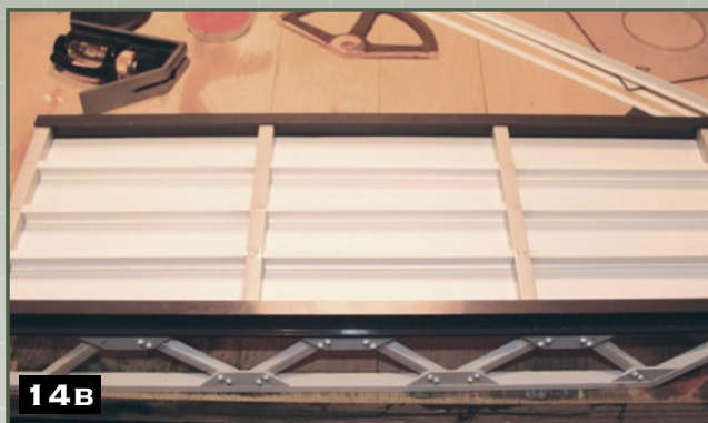
Step 14) Add braces and supports. Cut a piece of diamond plate plastic card and glue it onto the surface of the bridge. Turn the bridge over and glue small I-beams between each square box tube.
