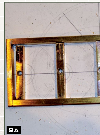
Step 9) Solder brass box tube sections. Lay the brass box tube sections and the rectangle piece over the drawing to locate where the pieces need to go. Solder them in place. Complete four sections.
