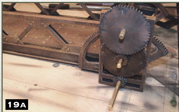
Step 19) Paint and glue the gears. Paint the gears in the same fashion and fit them to the bridge. The lower shaft should stick out from the bridge about 3" on the near side and 1" on the far side. Slide and glue small gears into place on the lower shaft, being careful to avoid getting glue on the gear towers. Slide and glue small gears onto the top shaft so that they line up with the large gears on the bridge. Paint and slide the two remaining gear towers into place.
