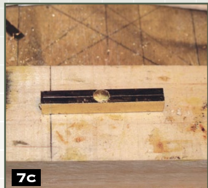
Step 7) Align and drill the box tubes. Cover two opposite sides of the box tube with black marker and draw a line down the center of the piece. Using a power drill, you will need to drill a hole on each side of the box tube. Make sure the holes line up with each other exactly, then drill one hole at a time. Do not try to drill all the way through from one side to the other, as the holes will not line up properly.
