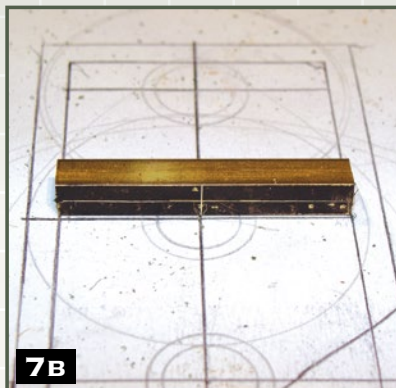
Step 7) Align and drill the box tubes. Cover two opposite sides of the box tube with black marker and draw a line down the center of the piece. Using a power drill, you will need to drill a hole on each side of the box tube. Make sure the holes line up with each other exactly, then drill one hole at a time. Do not try to drill all the way through from one side to the other, as the holes will not line up properly.
