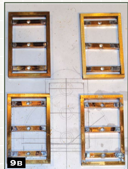
Step 9) Solder brass box tube sections. Lay the brass box tube sections and the rectangle piece over the drawing to locate where the pieces need to go. Solder them in place. Complete four sections.
