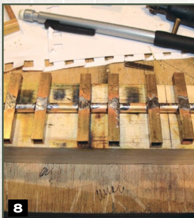
Step 8) Solder square tube pieces to the brass tube. Slide several pieces of square tube over a piece of brass tube. (This brass tube will be fit to your solid brass rod piece.) I chose to do six pieces of square tube at once to ensure the brass box tube section remained square during soldering. Solder the pieces to the tube, cut them off, and sand the brass tube flush.
