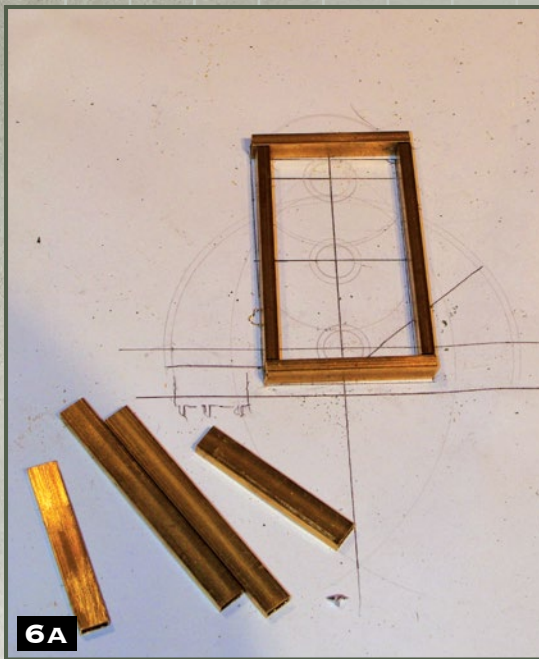
Step 6) Assemble the box frame. Once the rectangle pieces are assembled, measure sections of the square brass box tube so that they will fit inside the rectangle.
