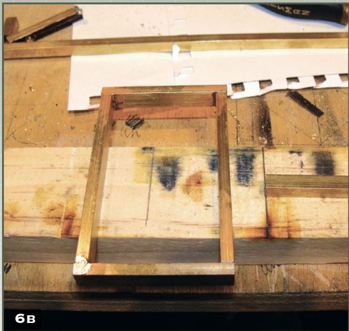
Step 6) Assemble the box frame. Once the rectangle pieces are assembled, measure sections of the square brass box tube so that they will fit inside the rectangle.
