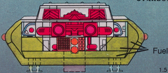
STARBOARD CUTAWAY
