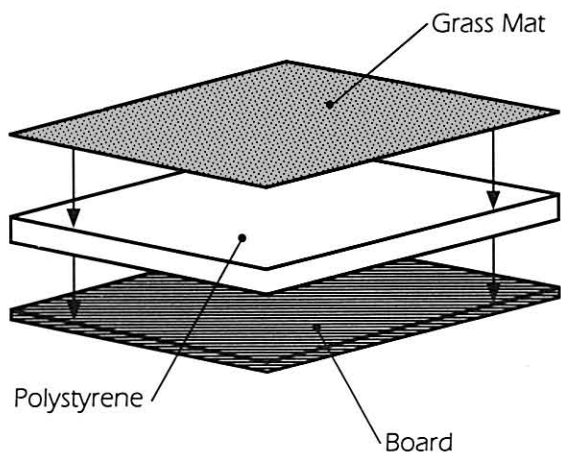
DIAGRAM 31 Panel Construction
