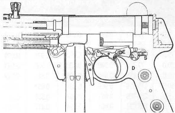
Walther MP-K with stock folded
